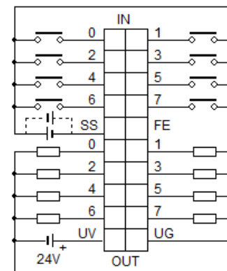
iR-DM16-P
